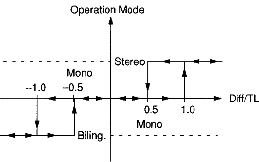
Fig. 3-6: Hysteresis loop for operation mode determination
